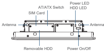
Front I/O
