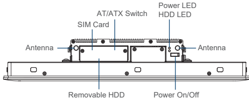
Front I/O
