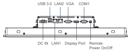
Rear I/O
