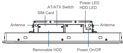
Front I/O
